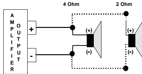
PARALLEL CONNECTION USING 4 OHM SPEAKERS
