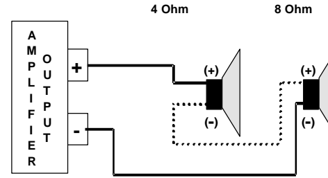
SERIES CONNECTION USING 4 OHM SPEAKERS
